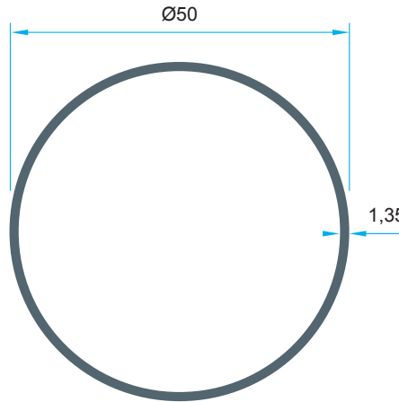
Code: P-1334 0,558 kg/m
