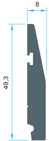
Code: P-1137 0,835 kg/m
