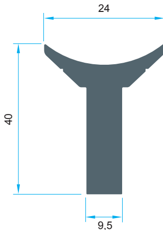
Code: P-1226 1,182 kg/m
