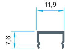
Code: AL6505 0,068 kg/m
