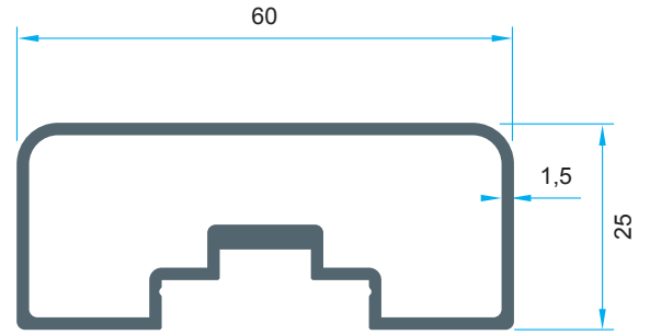
Code: P-1072 0,783 kg/m
