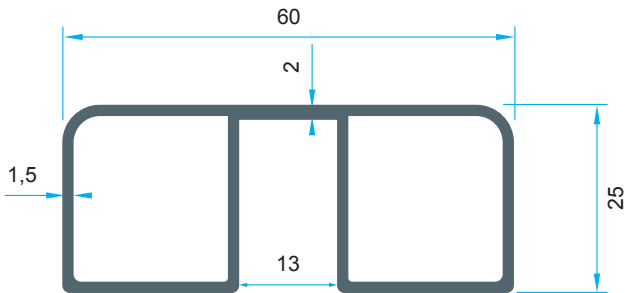
Code: P-1126 0,794 kg/m
