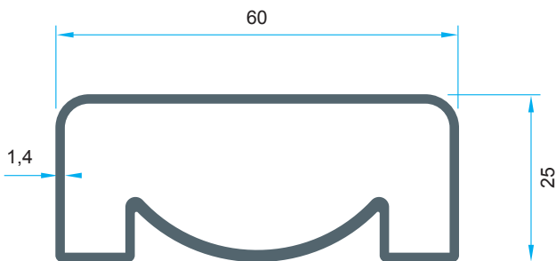
Code: P-1321 0,729 kg/m
