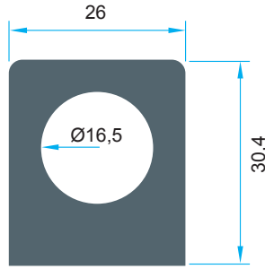
Code: P-1119 1,558 kg/m
