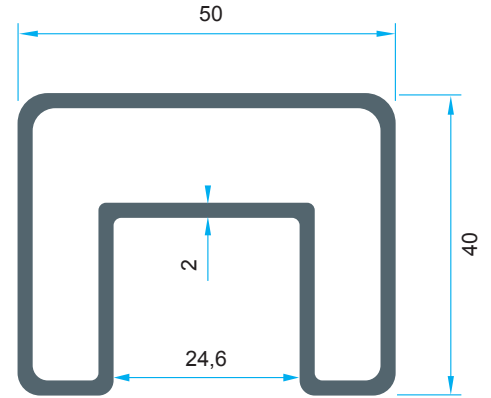
Code: P-1032 1,168 kg/m
