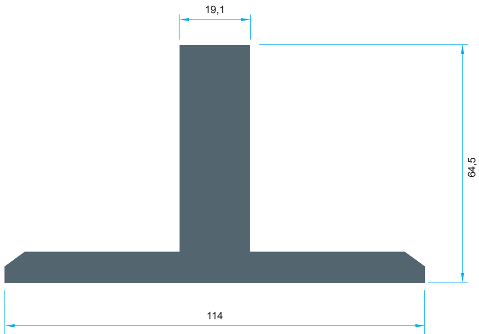
Code: P-1016 5,465 kg/m
