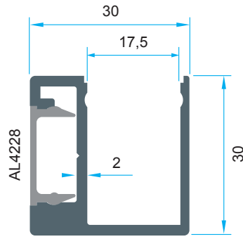
Code: P-1068 0,610 kg/m
