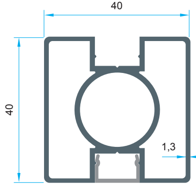
AL6505 Code: P-1067 0,905 kg/m
