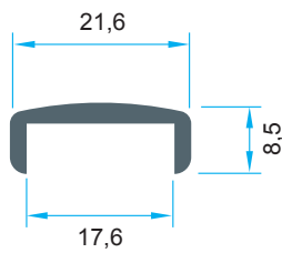
Code: AL6728 0,178 kg/m
