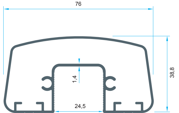
Code: AL6948 1,013 kg/m
