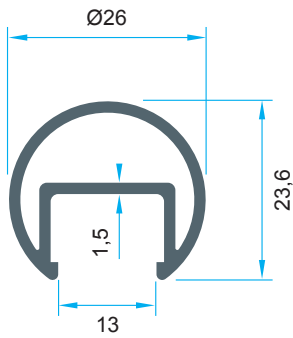
Code: AL7619 0,404 kg/m
