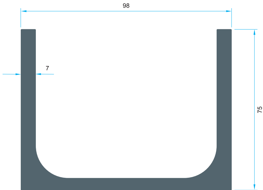
Code: P-1268 4,428 kg/m
