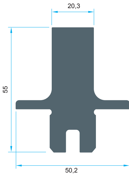
Code: P-1236 3,041 kg/m
