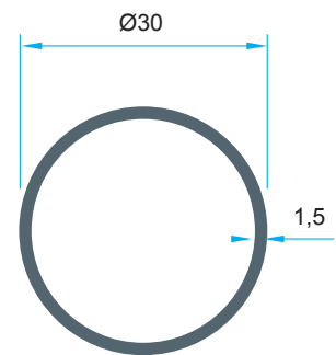
Code: P-1546 0,364 kg/m
