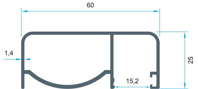
Code: P-1319 0,694 kg/m
