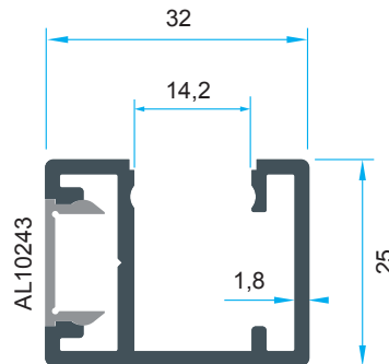
Code: P-1631 0,547 kg/m
