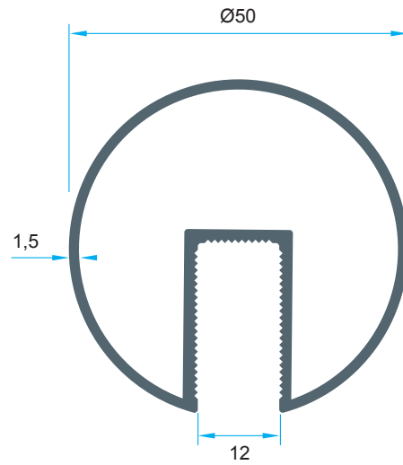
Code: AL7798 0,872 kg/m
