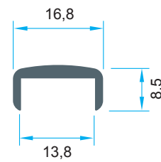
Code: AL7426 0,141 kg/m
