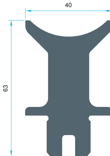
Code: P-1234 3,428 kg/m
