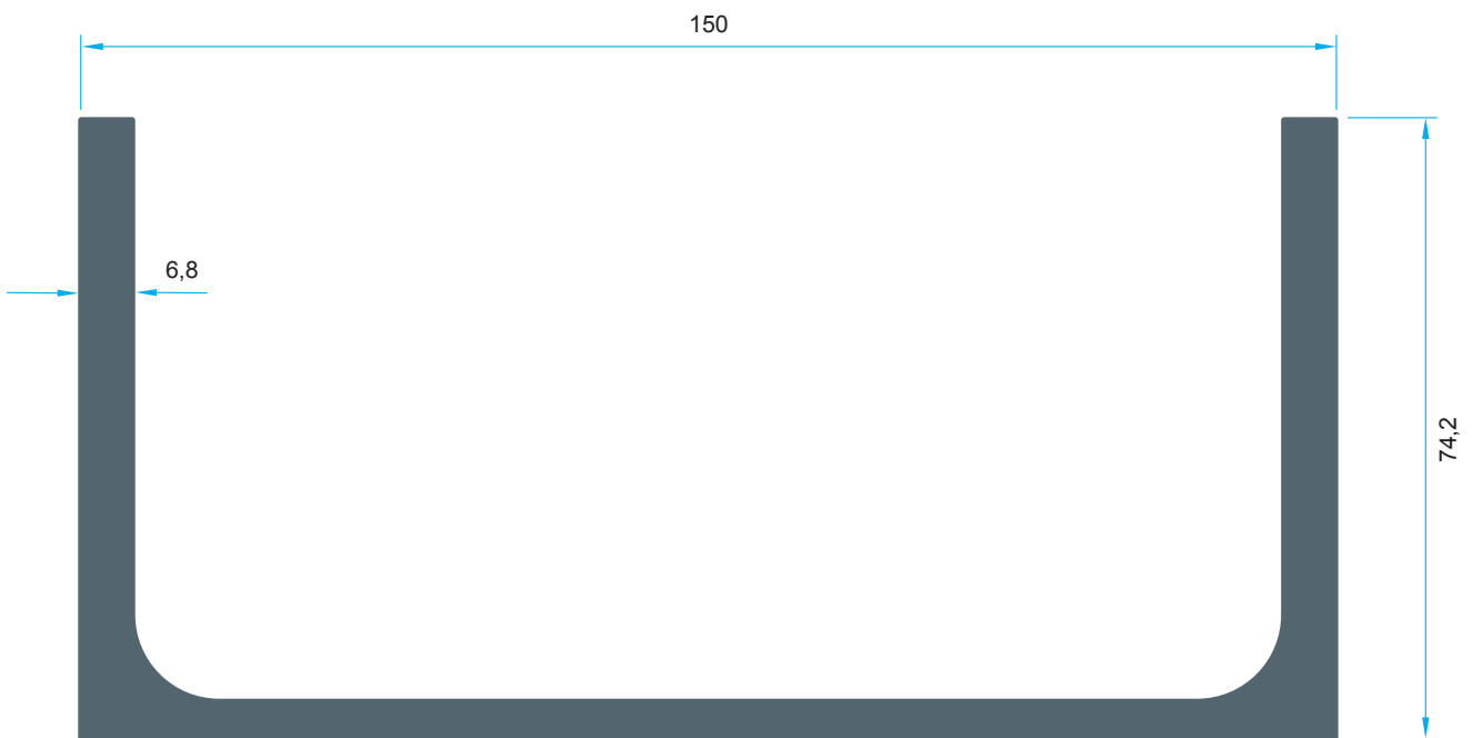
Code: P-1224 4,699 kg/m
