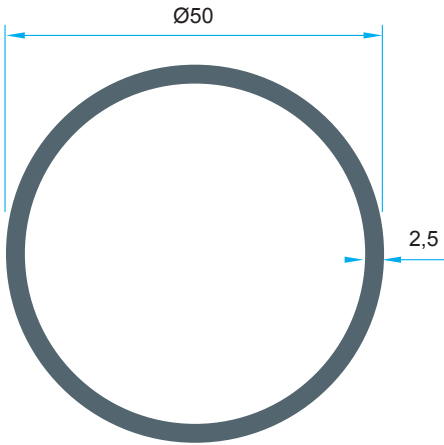
Code: P-1388 1,011 kg/m
