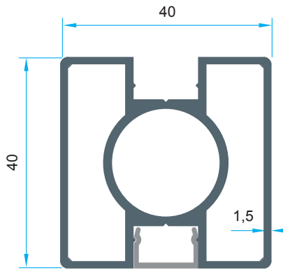
AL6505 Code: P-1633 1,027 kg/m
