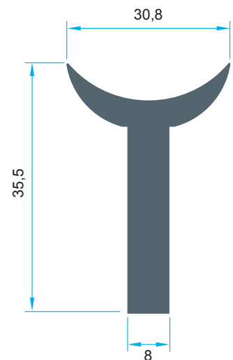
Code: P-1254 1,183 kg/m
