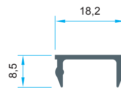
Code: AL4228 0,123 kg/m
