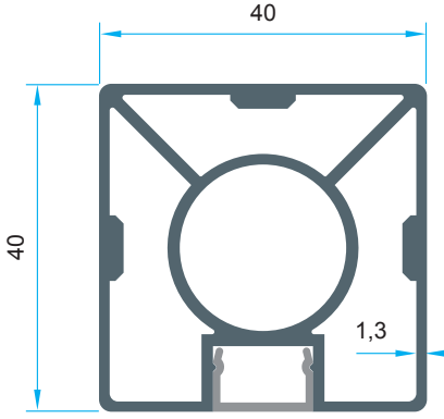
AL6505 Code: P-1057 1,090 kg/m
