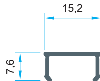
Code: AL9958 0,084 kg/m
