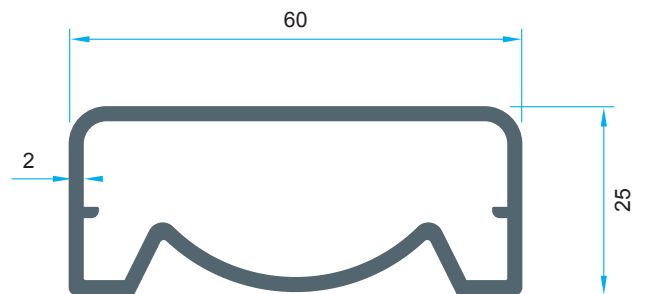
Code: P-1634 0,943 kg/m
