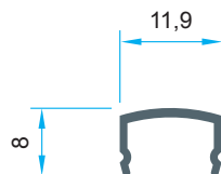
Code: AL2647 0,067 kg/m
