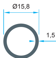
Code: P-1146 0,182 kg/m
