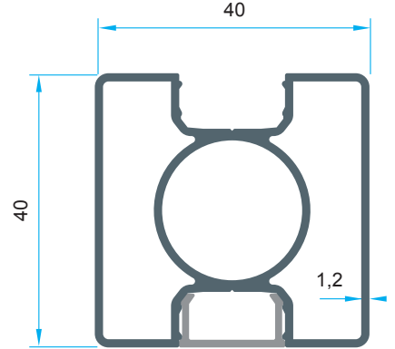
AL9958 Code: P-1317 0,799 kg/m
