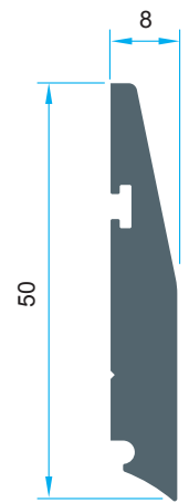
Code: P-1140 0,821 kg/m
