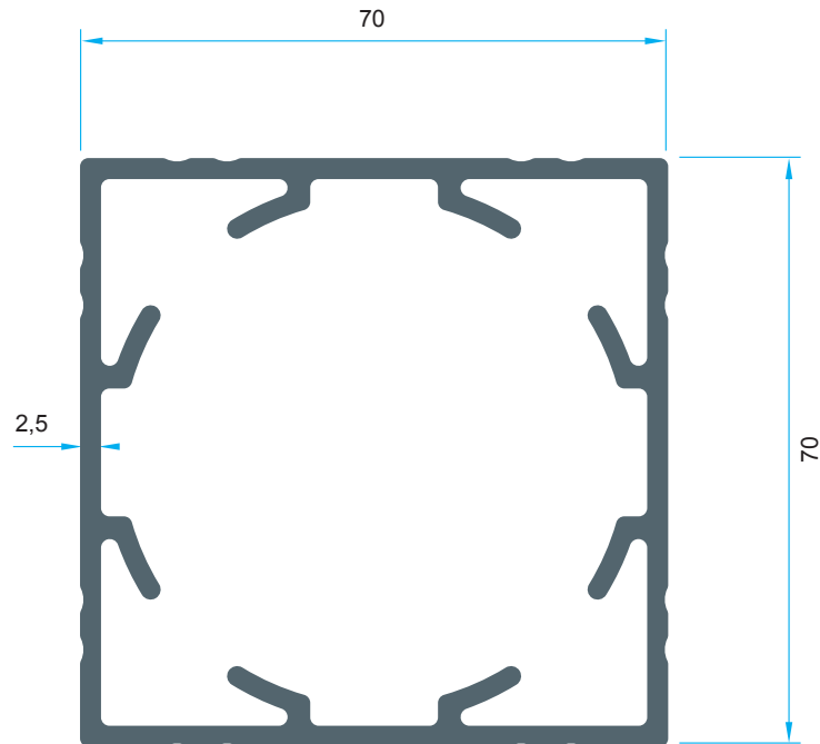
Code: P-1638 2,425kg/m
