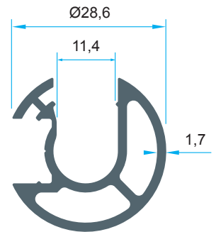
Code: P-1118 0,571 kg/m
