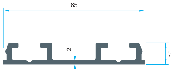
Code: P-1602 0,640 kg/m
