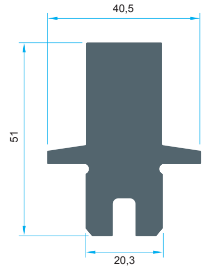
Code: P-1235 2,836 kg/m
