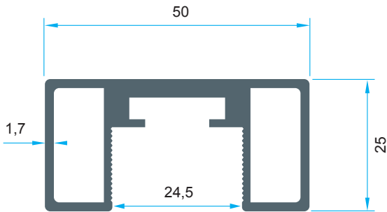
Code: P-1523 0,964 kg/m
