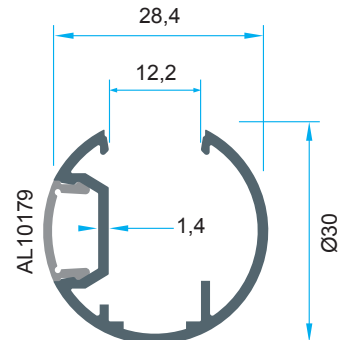
Code: P-1592 0,359 kg/m
