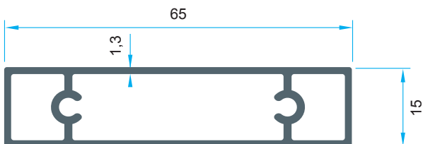
Code: P-1603 0,698 kg/m
