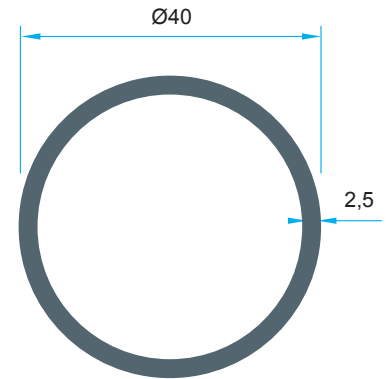
Code: P-1560 0,798 kg/m
