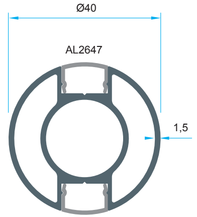
Code: P-1087 0,815 kg/m
