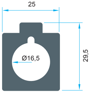
Code: P-1065 1,214 kg/m
