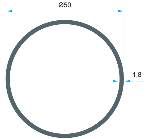
Code: P-1346 0,739 kg/m
