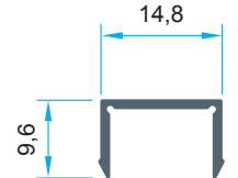
Code: AL7588 0,098 kg/m
