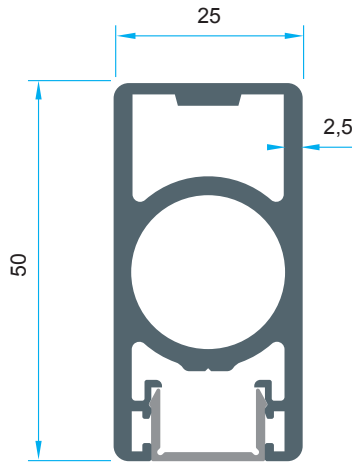
AL7588 Code: P-1238 1,200 kg/m
