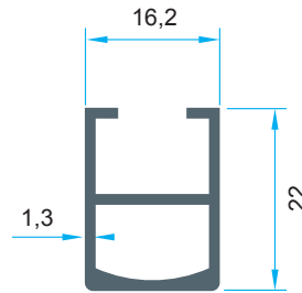
Code: P-1635 0,284 kg/m
