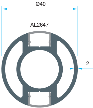
Code: P-1054 1,163 kg/m
