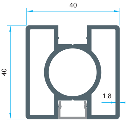
AL6505 Code: P-1632 1,187 kg/m
