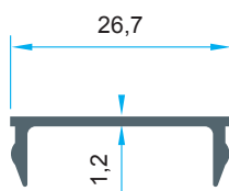
Code: AL10143 0,145 kg/m
