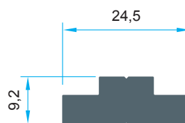
Code: P-1229 0,477 kg/m
