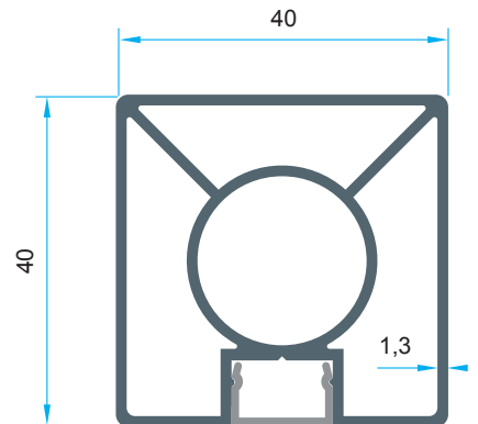
AL6505 Code: P-1401 0,934 kg/m
