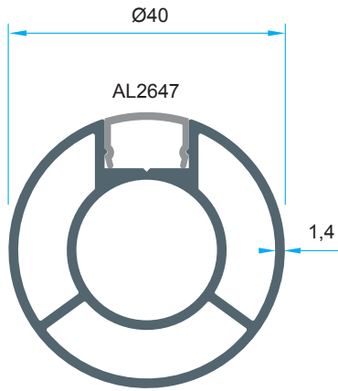
Code: P-1387 0,814 kg/m
