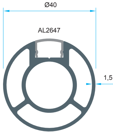
Code: P-1073 0,976 kg/m
