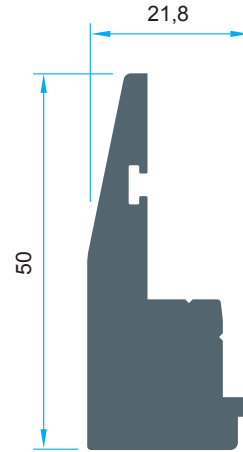
Code: P-1138 1,477 kg/m
