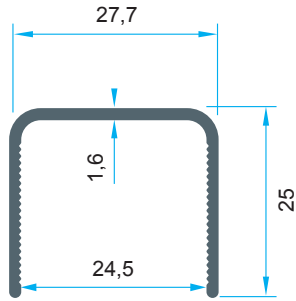
Code: P-1031 0,295 kg/m
