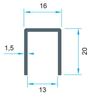
Code: AL8093 0,214 kg/m
