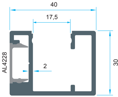
Code: P-1056 0,791 kg/m
