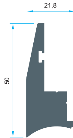
Code: P-1139 1,293 kg/m
