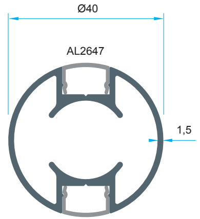
Code: P-1591 0,747 kg/m
