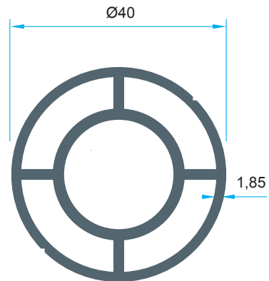
Code: P-1266 1,128 kg/m
