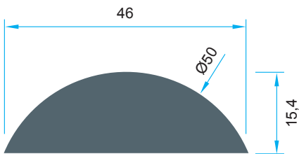
Code: P-1028 1,393 kg/m
