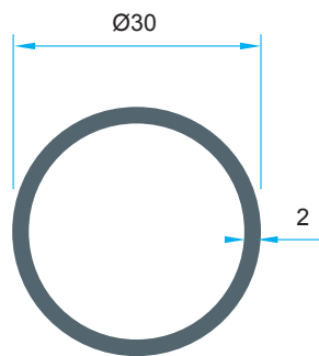
Code: P-1074 0,477 kg/m
