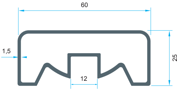
Code: P-1327 0,799 kg/m
