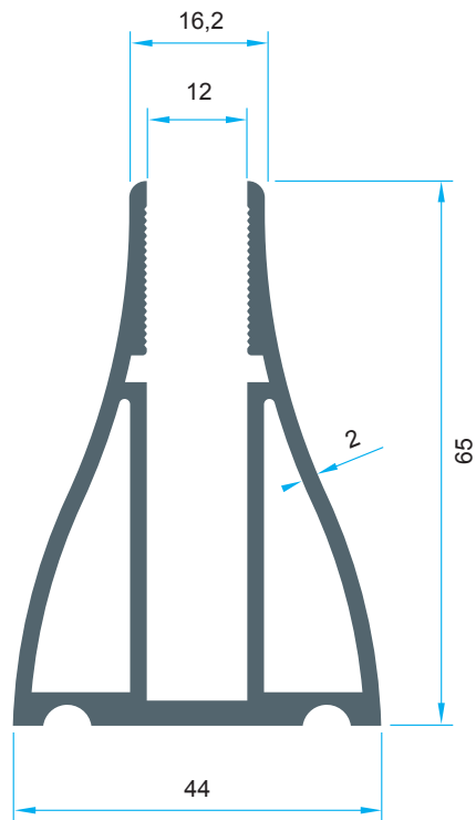
Code: P-1082 1,525 kg/m
