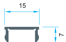
Code: AL10243 0,086 kg/m
