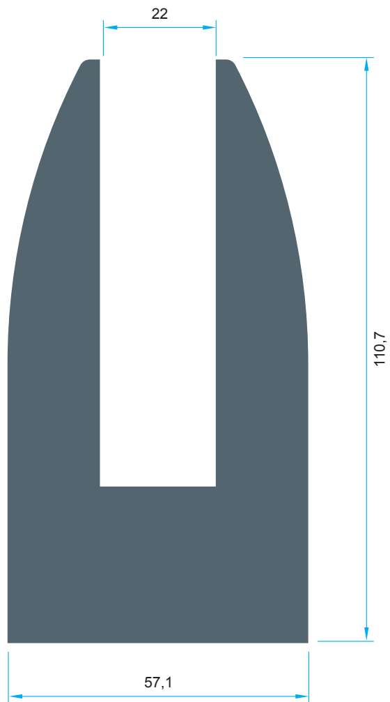
Code: P-1017 10,835 kg/m
