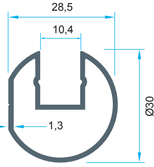
Code: P-1322 0,412 kg/m
