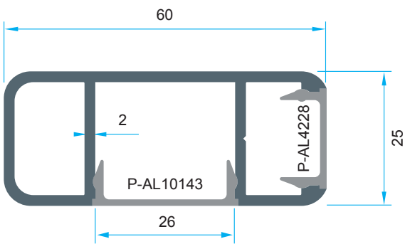
Code: P-1108 0,844 kg/m
