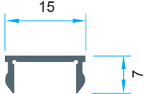
Code: P-AL10243 0,086 kg/m
