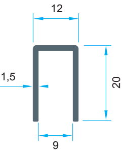
Code: P-AL8092 0,198 kg/m
