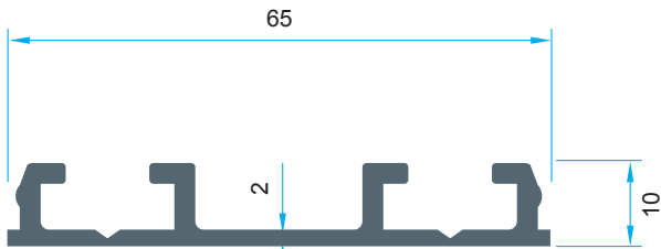
Code: P-1602 0,640 kg/m
