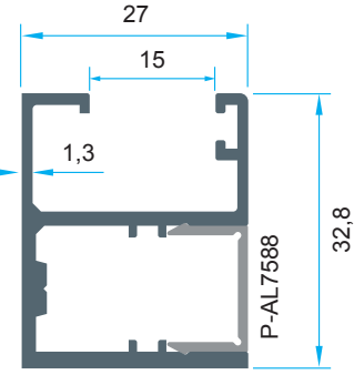
Code: P-1075 0,531 kg/m
