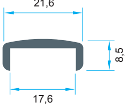
Code: P-AL6728 0,178 kg/m
