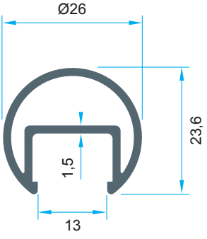
Code: P-AL7619 0,400 kg/m
