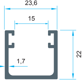
Code: P-1400 0,351 kg/m
