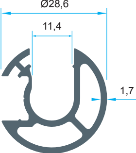
Code: P-1118 0,571 kg/m
