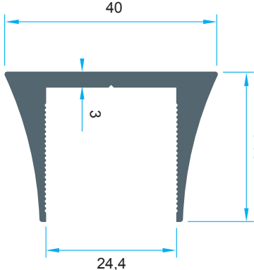
Code: P-1537 0,734 kg/m
