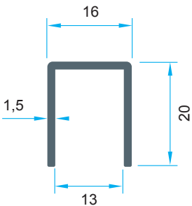
Code: P-AL8093 0,214 kg/m
