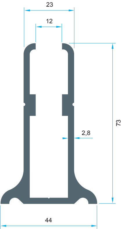
Code: P-1357 1,741 kg/m
