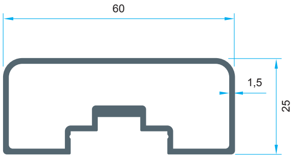
Code: P-1072 0,783 kg/m
