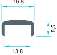
Code: P-AL7426 0,141 kg/m
