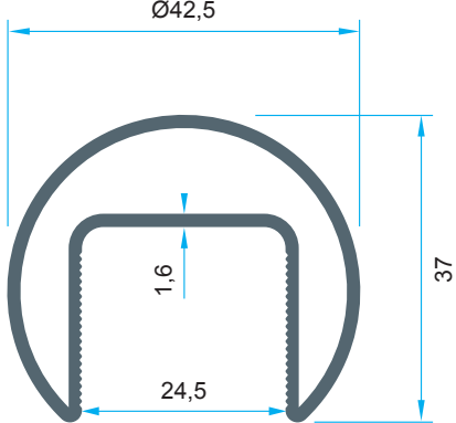
Code: P-1030 0,721 kg/m
