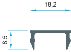
Code: P-AL4228 0,123 kg/m
