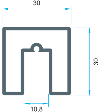
Code: P-AL6528 0,628 kg/m
