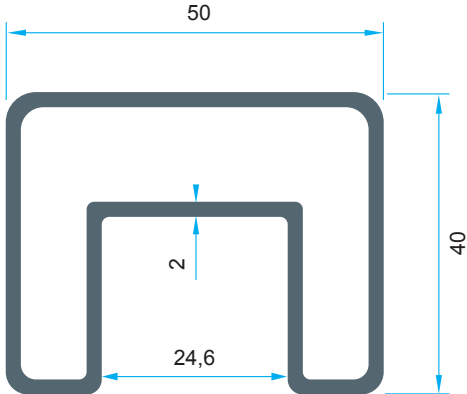
Code: P-1032 1,168 kg/m
